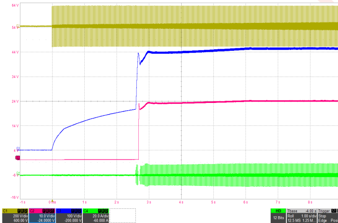
Figure 3: Typical startup waveform with 600µF hold-up capacitor (115Vrms, 60Hz) Ch1: V_{in} (200V/div), Ch2: V_{out} (10V/div), Ch3: Hold-up capacitor voltage (100V/div), Ch4: I_{in} (20A/div), Timebase: (1s/div).
