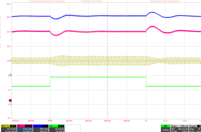
Figure 5: Load transient with 600µF hold-up capacitor (50%-75%-50% of I_{max} , 115Vrms, 60Hz) Ch1: I_{in} (20A/div), Ch2: V_{out} (5V/div), Ch3: Hold-up capacitor voltage (100V/div), Ch4: I_{out} (10A/div), Timebase: (200ms/div).
