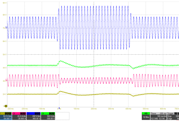
Figure 7: Input transient with 600µF hold-up capacitor at full load (115Vrms-220Vrms-115Vrms, 60Hz) Ch1: Vout (10V/div), Ch2: Iin (20A/div), Ch3: Vin (200V/div), Ch4: Vhold-up (100V/div), Timebase: (100ms/div).
