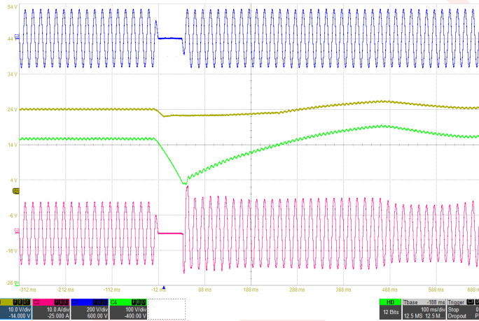
Figure 9: Line drop out with 600µF hold-up capacitor at full load (115Vrms, 60Hz) Ch1: Vout (10V/div), Ch2: Iin (10A/div), Ch3: Vin (200V/div), Ch4: Vhold-up (100V/div), Timebase: (100ms/div).
